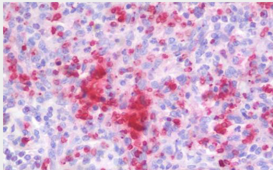
Anti-TGFB1 / TGF Beta 1 antibody IHC staining of human spleen.
